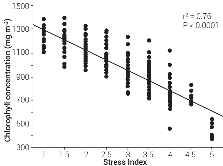
Figure 2. Relationship between needle chlorophyll concentration (mg m -2 ) and the stress index in Abies religiosa seedlings planted on the field at 3460 m of altitude, Monarch Butterfly Biosphere Reserve, ejido La Mesa, State of Mexico.
